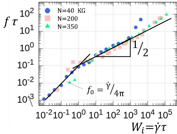
Fig.1 Dimensionless rotation frequency as functions of Weissenberg number
