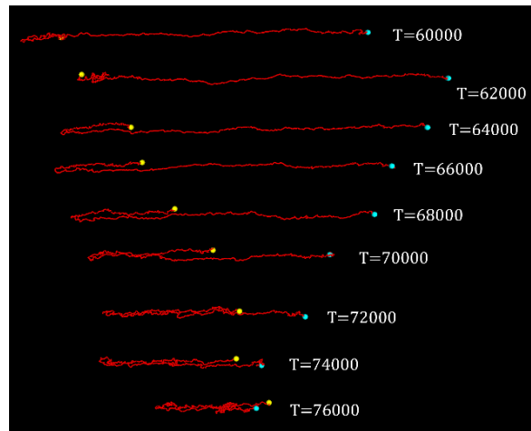
Fig.3 Snapshots of a rotating chain. N = 350, W_i = 3 \times 10^3
